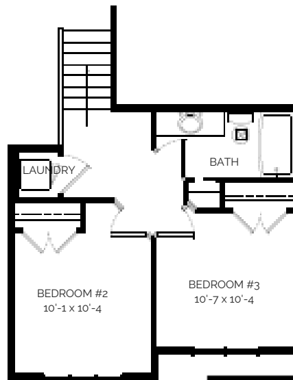
Upper Floor 421 Sq Ft
