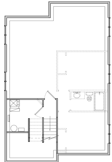
UNDEVELOPED BASEMENT
