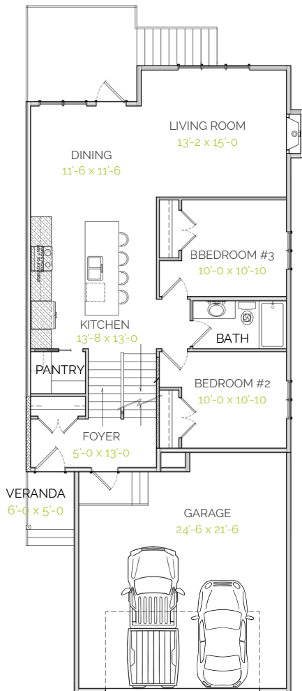
MAIN FLOOR 1092 SQ. FT.
