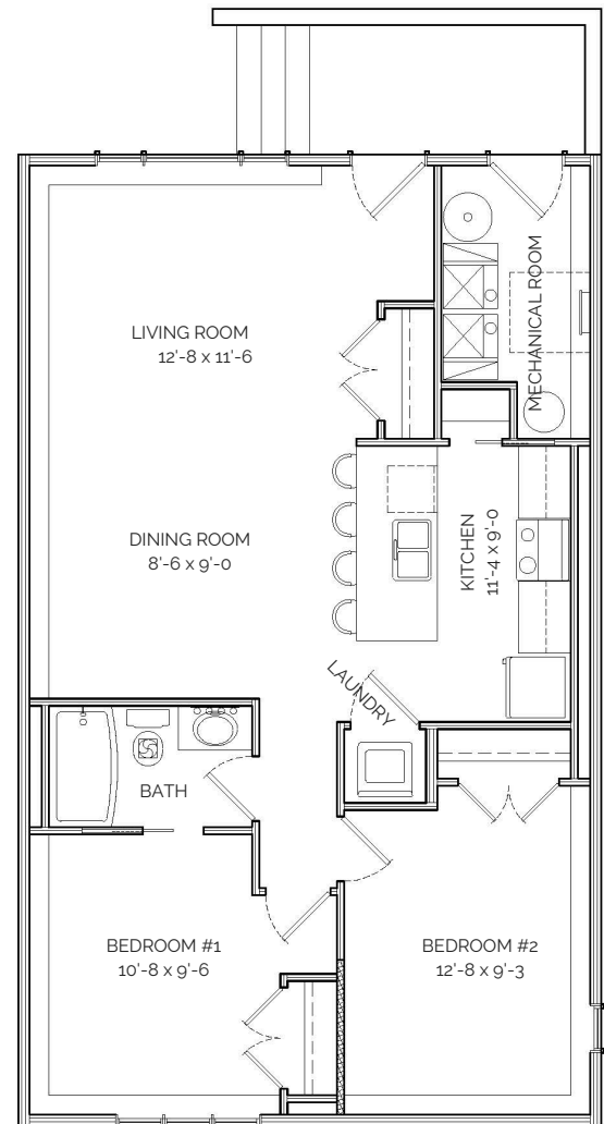
Lower Floor Suite 890 Sq Ft
