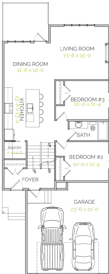
MAIN FLOOR 1118 SQ. FT.
