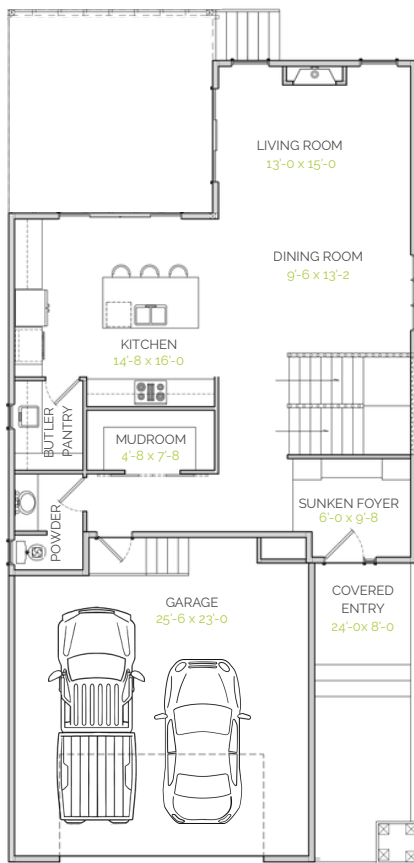
MAIN FLOOR 1044 SQ. FT.
