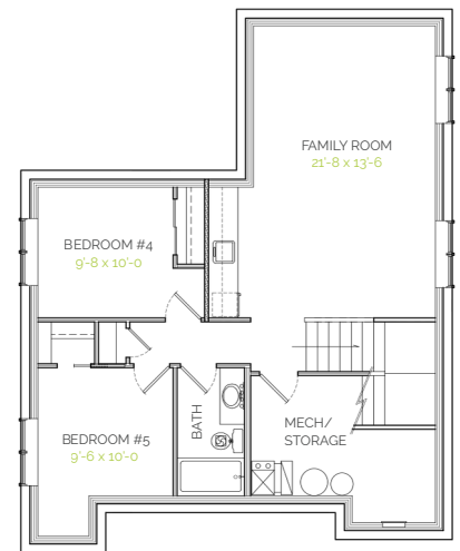
BASEMENT 831 SQ. FT.
