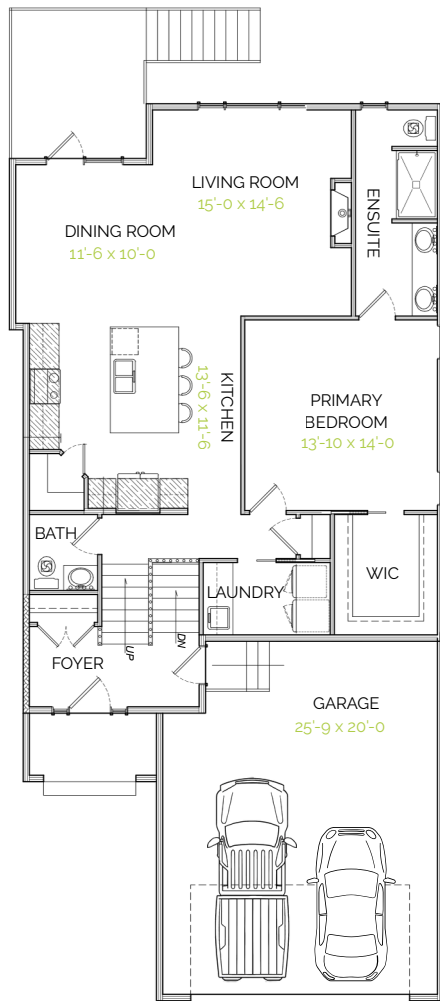
MAIN FLOOR 1253 SQ. FT.
