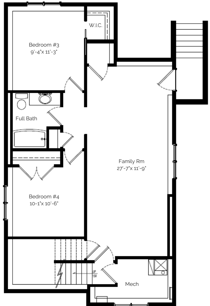
Lower Floor 843 Sq Ft
