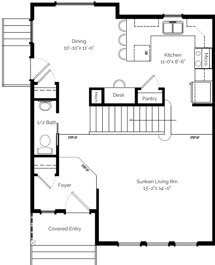
Main Floor 640 Sq Ft
