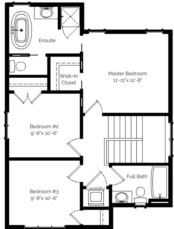
Upper Floor 734 Sq Ft
